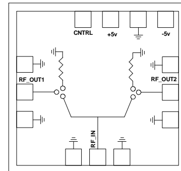
Functional Diagram
